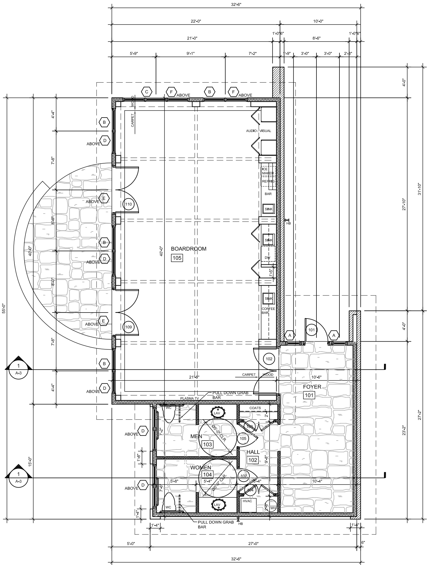
1 FLOOR PLAN
